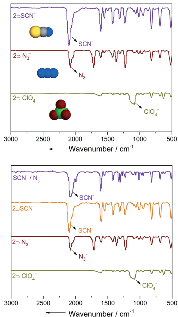
Fig. 3 FTIR spectra of compound 2 and its various anion exchanged products with highlighted bands of corresponding anions (top). FTIR spectra of different binary mixtures of anions of compound 2 (bottom).
