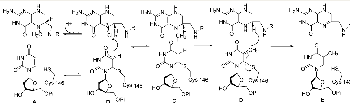
Scheme 1 (a) Mechanism of TSase-catalyzed conversion of dUMP to dTMP.
