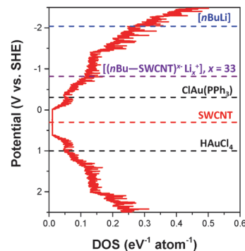
Fig. 4 The averaged DOS of the (n,m) distribution in a HiPco sample was derived from ref. 13 and 22. The averaged DOS comprises 28 semi-conducting and 18 metallic SWCNTs as identified from resonance Raman spectroscopy. 23 For simplicity, all (n,m) -SWCNTs equally contribute to the DOS, although, as in a typical SWCNT sample the proportion of semi-conducting:metallic SWCNTs is adjusted to 2:1. The position of the Fermi level, E_F , of undoped HiPco SWCNTs was determined from cyclic voltammetry ( \sim +0.30 V vs. SHE), although in principle, the E_F will vary for each (n,m) -SWCNT. 1,24
