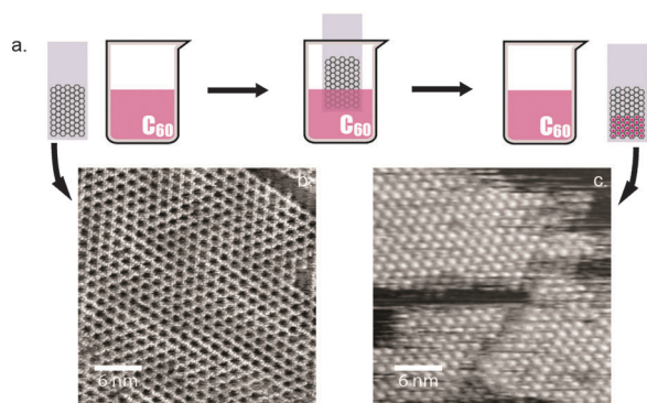
Fig. 3 Schematic illustration of dipstick preparation of COF-1/fullerene H/G structure. The image in (b) shows the as-synthesized COF-1 on HOPG. Following immersion into a solution of C_{60} in heptanoic acid (a) and subsequent drying, STM images like that in (c) reveal COF-1 populated with C_{60} guest molecules. Imaging parameters: voltage U_t = -800 mV, tunneling current I = 100 pA.
