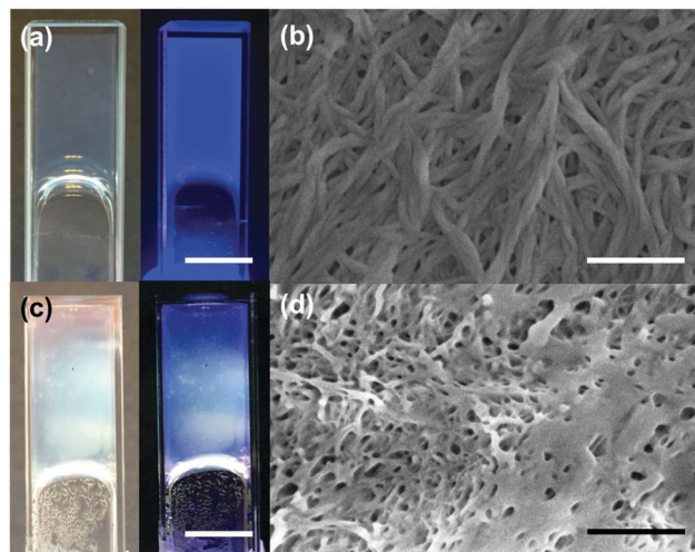
Fig. 2 Gels formed using GdL before irradiation (a) photographed under natural light (left) and under UV light (right), scale bar represents 1 cm. (b) SEM image of GdL gel, scale bar represents 500 nm. Gels formed by GdL after irradiation for 2 hours (c) photographed under natural light (left) and under UV light (right), scale bar represents 1 cm. (d) SEM image after irradiation, scale bar represents 500 nm.
