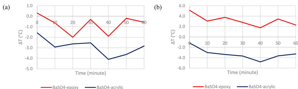
Fig. 8 Surface temperature difference with ambient temperature of (a) \text{BaSO}_4 -epoxy paint and \text{BaSO}_4 -acrylic paint with DMF as the solvent. (b) \text{BaSO}_4 -epoxy paint and \text{BaSO}_4 -acrylic paint with water as the solvent.
