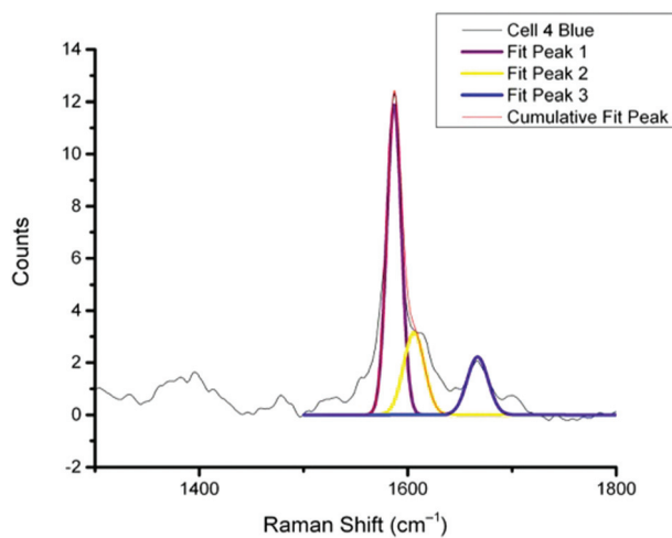
Fig. 4 Representative example of peak fitting for a multiplex spectrum generated from k -means cluster analysis (cell 4 blue cluster). Peaks were fitted using a GaussAmp function with constrained parameters resulting in the 3 individual peak fits, Fit 1, 2 and 3 and the overall resultant Cumulative Fit Peak shown overlaid on the original spectrum (black line).
