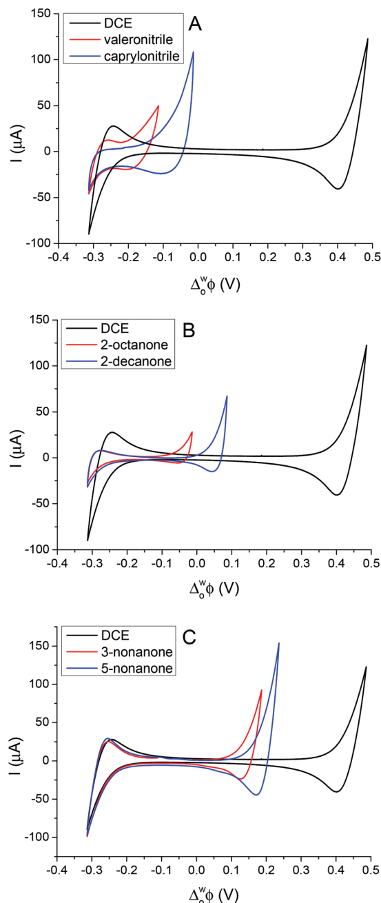
Fig. 1 Comparison of the potential windows obtained at lower density organic/water interfaces with the DCE/water interface: valerionitrile, caprylonitrile (A); 2-octanone, 2-decanone (B); 3-nonanone, 5-nonanone (C) for cell 1, scan rate: 50 mV s -1 .
