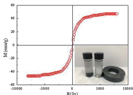
Fig. 8 Magnetization curve of Fe 3 O 4 @-SiO 2 -g-PAMAM-AO; the inset shows a photograph of Fe 3 O 4 @-SiO 2 -g-PAMAM-AO dispersion in ethanol and its magnetic response when placed in an external magnetic field (right).
