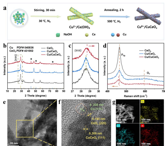
Fig. 2 (a) Synthetic route of the Cu/CuCeO x catalyst by a coprecipitation method. (b) XRD spectra, (c) local amplification of (111) and (d) Raman spectra for \text{CeO}_x , Cu/ \text{CeO}_x , and Cu/CuCeO x catalysts ( \text{CeO}_2 , yellow, PDF# 43-1002; Cu, blue, PDF# 04-0836). (e and f) HRTEM images and (g) EDX elemental distribution mapping images of Cu/CuCeO x .
