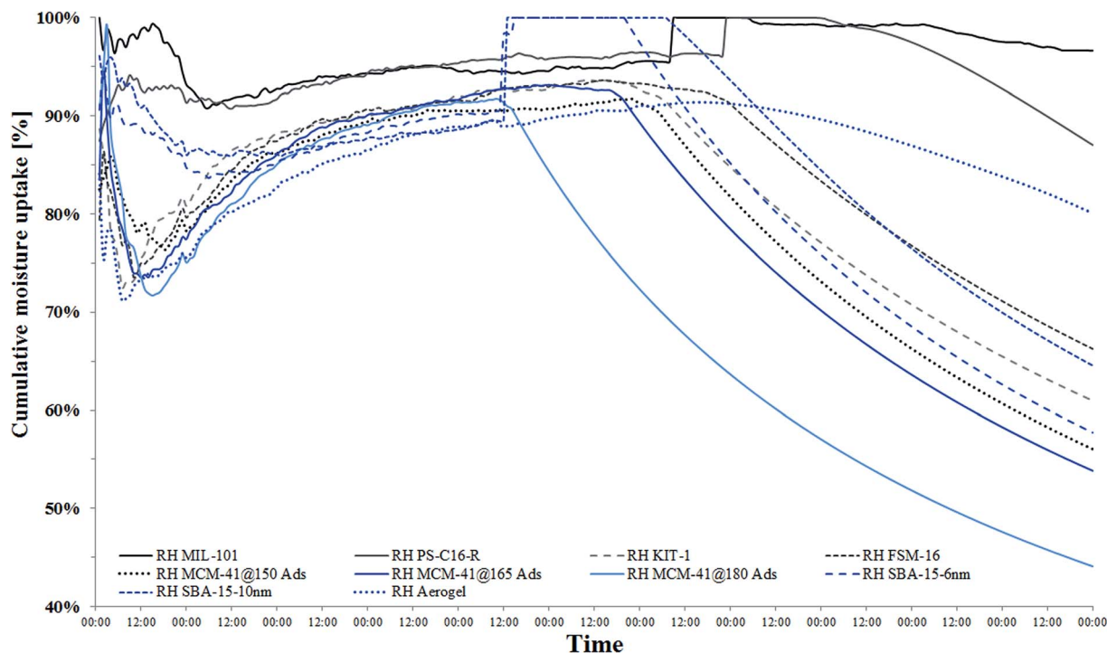
Fig. 4 Cumulative water vapour uptake for all desiccant candidates. Initial w = 0 for all desiccant materials and the moisture load applied is the moisture content of the infiltrated air at ACH = 0.35^{-1} , where \phi_e = 0.95 .
