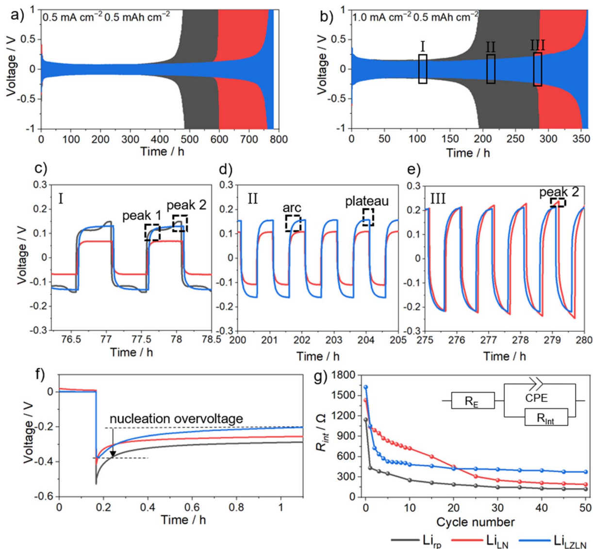
Fig. 4 Galvanostatic cycling of symmetric \text{Li}_{\text{rp}}||\text{Li}_{\text{rp}} (grey), \text{Li}_{\text{LN}}||\text{Li}_{\text{LN}} (red) and \text{Li}_{\text{LZLN}}||\text{Li}_{\text{LZLN}} (blue) cells at a fixed current density of (a) 0.5 \text{ mA cm}^{-2} and (b) 1.0 \text{ mA cm}^{-2} with a capacity of 0.5 \text{ mA h cm}^{-2} . (c)–(e) Emphasizes the electrodeposition/-dissolution behavior from (b) of \text{Li}_{\text{rp}}||\text{Li}_{\text{rp}} , \text{Li}_{\text{LN}}||\text{Li}_{\text{LN}} and \text{Li}_{\text{LZLN}}||\text{Li}_{\text{LZLN}} after (c) 75, (d) 200 and (e) 275 cycles at a current density of 1.0 \text{ mA cm}^{-2} . (f) Nucleation overvoltage profiles from the first electrodeposition at 0.5 \text{ mA cm}^{-2} . (g) R_{\text{int}} evolution determined by EIS within the first 50 cycles at 0.5 \text{ mA cm}^{-2} .
