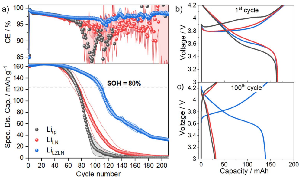
Fig. 6 (a) Electrochemical performance of NMC622||Li cells with \text{Li}_{\text{rp}} (grey), \text{Li}_{\text{LN}} (red) or \text{Li}_{\text{LZLN}} (blue) electrodes as negative electrode. (a) Capacity retention and the coulombic efficiency in a long-term cycling experiment at 0.2C. (b) The corresponding charge/discharge voltage profiles after initial cycle and (c) after 100 cycles.
