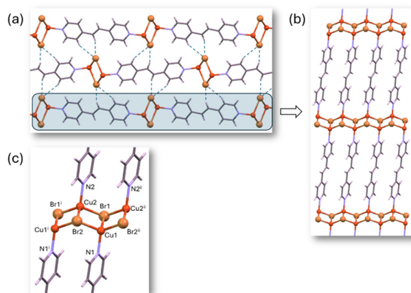
Fig. 5 (a) Crystal packing of compound 5b showing the hydrogen bonding interactions holding together the 2D planar sheets. (b and c) Detail of the 2D planar sheet showing the \text{CuBr} ladder-like chain connected by bridging BPEE ligands.
