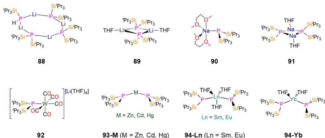
Fig. 25 P^{\dagger\dagger} complexes \{Li(\mu-P^{\dagger\dagger})_3\{Li[\mu-P(Si^iPr_3)H]\}\} ( 88 ), [Li(\mu-P^{\dagger\dagger})(THF)]_2 ( 89 ), [Na(P^{\dagger\dagger})(DME)_2] ( 90 ), [Na(\mu-P^{\dagger\dagger})(THF)]_2 ( 91 ), [W(P^{\dagger\dagger})(CO)_5][Li(THF)_4] ( 92 ), [M(P^{\dagger\dagger})_2] ( 93-M ; M = Zn, Cd, Hg), [Ln(P^{\dagger\dagger})_2(THF)_3] ( 94-Ln ; Ln = Sm, Eu), [Yb(P^{\dagger\dagger})_2(THF)_2] ( 94-Yb ).
