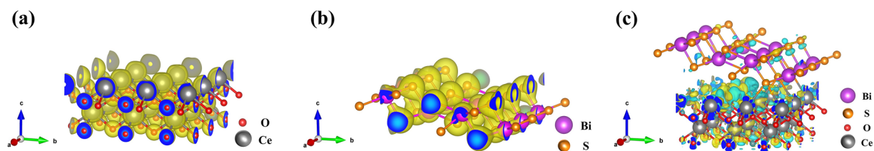
Fig. 9 Charge distribution of (a) CeO 2 and (b) Bi 2 S 3 before contacting (c) difference in charge density of CeO 2 /Bi 2 S 3 .
