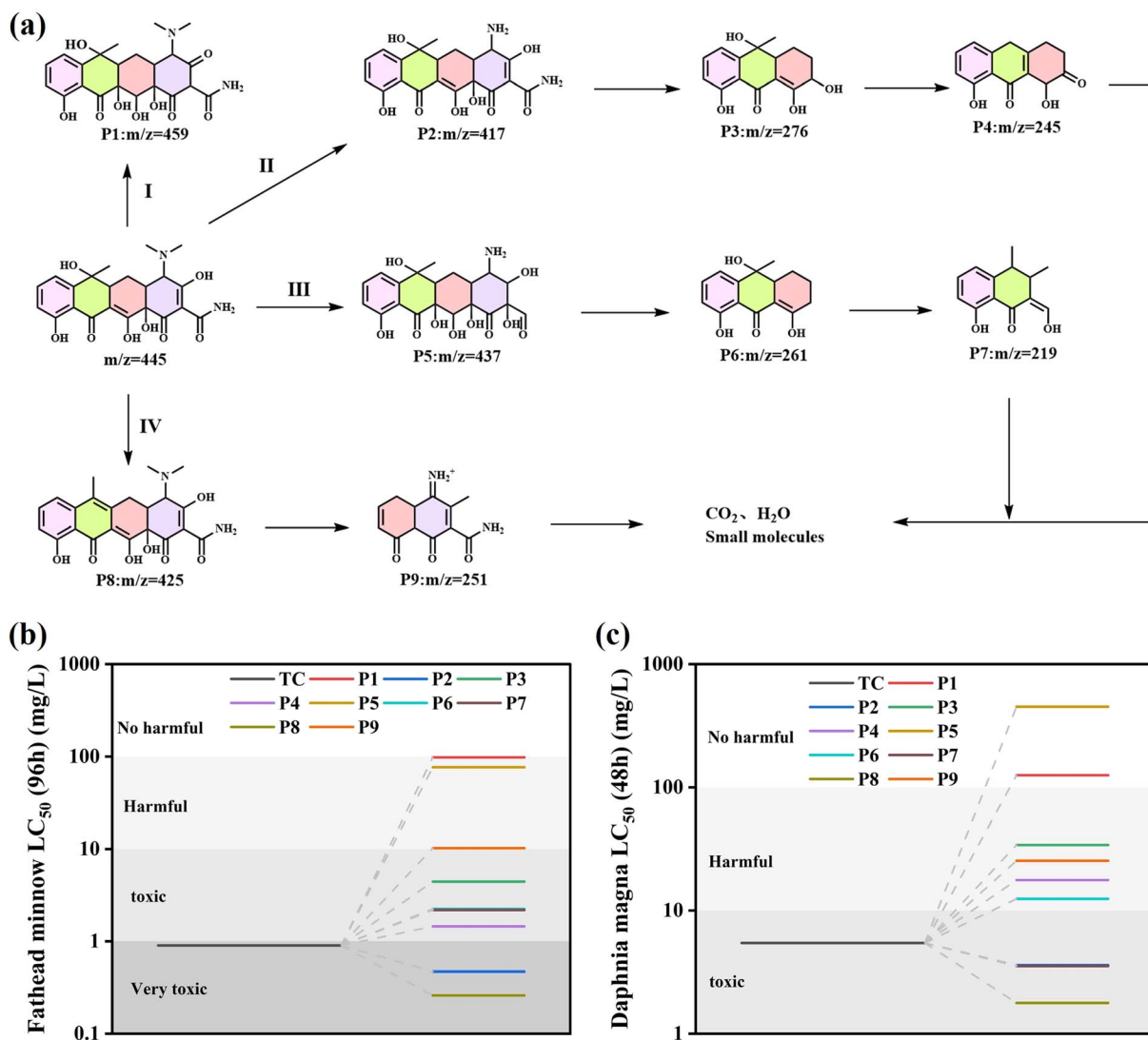
Fig. 11 (a) Possible intermediates and pathways for TC degradation by CeO 2 /Bi 2 S 3 -2 photocatalysts; (b) fathead minnow LC 50 (96 h); (c) Daphnia magna LC 50 (48 h).
