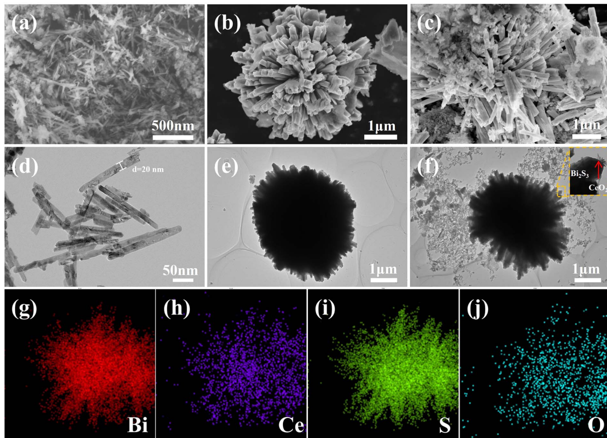
Fig. 2 SEM images of (a) \text{CeO}_2 ; (b) \text{Bi}_2\text{S}_3 ; (c) \text{CeO}_2/\text{Bi}_2\text{S}_3 -2, TEM images of (d) \text{CeO}_2 ; (e) \text{Bi}_2\text{S}_3 ; (f) \text{CeO}_2/\text{Bi}_2\text{S}_3 -2; EDS elemental distribution mapping of (g) Bi; (h) Ce; (i) S; (j) O in \text{CeO}_2/\text{Bi}_2\text{S}_3 -2.
