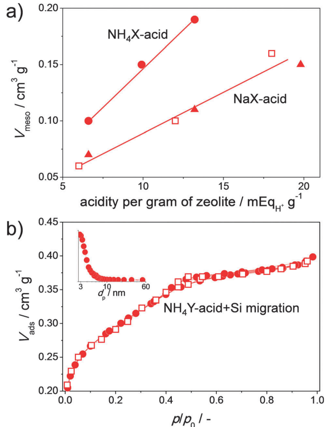
Fig. 7 Similarities between the porous properties of hierarchical X (a) and Y (b) zeolites prepared using different strategies. The 'NH 4 ' and 'Na' indicate the charge-balancing counter cations (CBCCC) present in the parent zeolites. (a) Comparison between the mesopore volumes ( V_{\text{meso}} ) or hierarchical X zeolites prepared by acid treatment (solid symbols, strategy Fig. 2b) 23 and those prepared by sequential acid and base treatment in presence of CTABr (open symbols, strategy Fig. 2c). 50 (b) Comparison between the nitrogen isotherms of hierarchical Y zeolites prepared by controlled acid treatment (solid symbols, strategy Fig. 2j) 23 and prepared by acid treatment in the presence of P123 (empty symbols) 51 Both materials in (b) were obtained by acid treatment of the NH 4 Y zeolite at elevated temperatures for ca. 72 h. The inset in (b) displays the BJH adsorption pore size distribution. The isotherm of the hierarchical Y with solid symbols in (b) was shifted down by 0.18 \text{ cm}^3 \text{g}^{-1} . The similar porosities emphasize that organic additives are not required in the preparation of hierarchical X and Y zeolites. (b, solid symbols) Reprinted with permission from Wiley-VCH Verlag.
