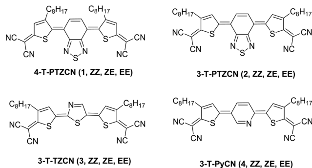
Fig. 25 Different heterocycle-based quinoïdal compounds.
