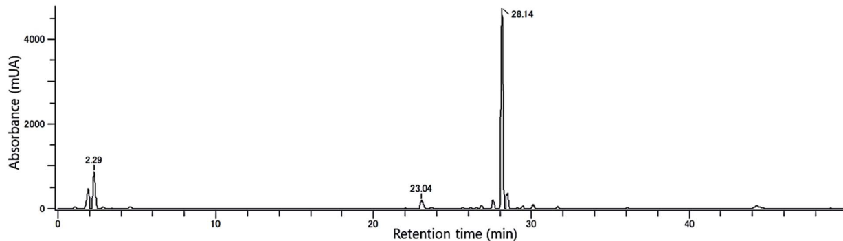
Scheme 2 (A) Biphase electrochemical synthesis of leuporelin, and (B) HPLC analysis of leuporelin (protected form, R. T. = 28.14) (5).
