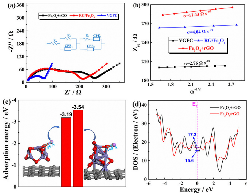
Fig. 25 (a) EIS plots of VGFC, RG/ \text{Fe}_3\text{O}_4 , and \text{Fe}_3\text{O}_4 + \text{rGO} and the corresponding equivalent circuit model (inset). (b) Z_{\text{re}} vs. \omega^{-1/2} curves of the three electrodes. (c) E_{\text{ad}} values of \text{Li}^+ on \text{Fe}_3\text{O}_4 + \text{rGO} and \text{Fe}_3\text{O}_4/\text{rGO} and the corresponding optimized configurations. (d) DOS of \text{Fe}_3\text{O}_4/\text{rGO} and \text{Fe}_3\text{O}_4 + \text{rGO} (the Fermi level is set to zero). Reproduced with permission. 276 Copyright 2021, American Chemical Society.
