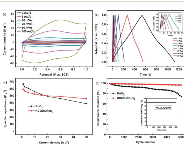
Fig. 27 (a) Cyclic voltammograms of RCQD/RuO 2 at different scan rates. (b) Charge-discharge curves of RCQD/RuO 2 at different current densities, and the inset shows a magnification at current densities of 10\text{--}50 \text{ A g}^{-1} . (c) Comparison of the specific capacitance change of RuO 2 and RCQD/RuO 2 as a function of current density. (d) Comparison of the cycling stability of the RuO 2 and RCQD/RuO 2 at a current density of 5 \text{ A g}^{-1} , and the inset shows the coulombic efficiency of RCQD/RuO 2 . Adapted with permission. 118 Copyright 2013, Royal Society of Chemistry.
