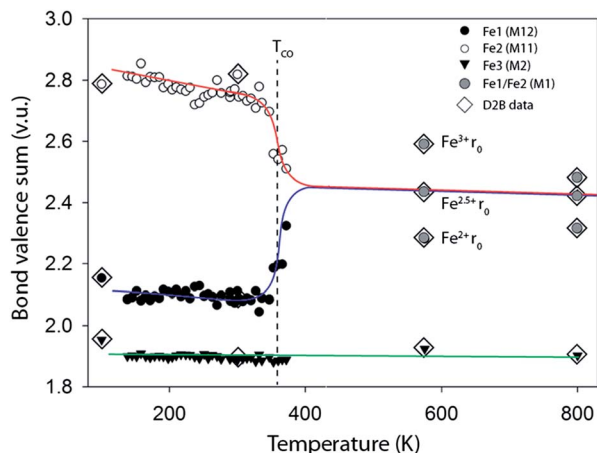
Fig. 3 Bond valence sums for the three transition metal sites in ilvaite calculated using the Fe^{3+} r_0 values for M11 and Fe^{2+} r_0 parameter for M12 and M2.† For the two high temperature data points in the orthorhombic phase where M11 is equivalent to M12, M1, with an average oxidation state of 2.5+ the BVS was calculated with Fe^{2+} , Fe^{2.5+} and Fe^{3+} r_0 values.
