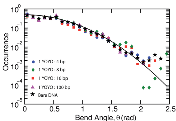
Fig. 6 Probability distribution of the DNA bending angle for angle \theta between tangents separated by the contour length of 20 nm for bare DNA (star), 1 YOYO per 100 base pairs (triangle), 1 YOYO per 16 base pairs (square), 1 YOYO per 8 base pairs (diamond), 1 YOYO per 4 base pairs (circle). The line is the wormlike chain prediction with the pre-determined persistence length of 56 nm in the case of bare DNA.
