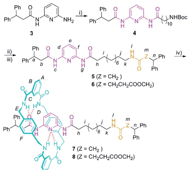
Scheme 2 Synthesis of the DAP-based threads 5 and 6 and the corresponding [2]rotaxanes 7 and 8 . Reagents and conditions: (i) 11-(tert-butoxycarbonylamino)undecanoic acid ( 9 ), DMAP, EDCI, CH 2 Cl 2 , 70%; (ii) TFA, CHCl 3 ; (iii) 3,3-diphenylpropanoic acid ( 10 ) or 2,2-diphenylethyl monosuccinate ( 11 ), DMAP, EDCI, CH 2 Cl 2 , 5 (39%); 6 (38%) (yields over two steps); (iv) isophthaloyl dichloride, p -xylylenediamine, Et 3 N, CHCl 3 ; 7 (Z = CH 2 ), 28%; 8 (Z = CH 2 CH 2 CO 2 CH 2 ), 23%.
