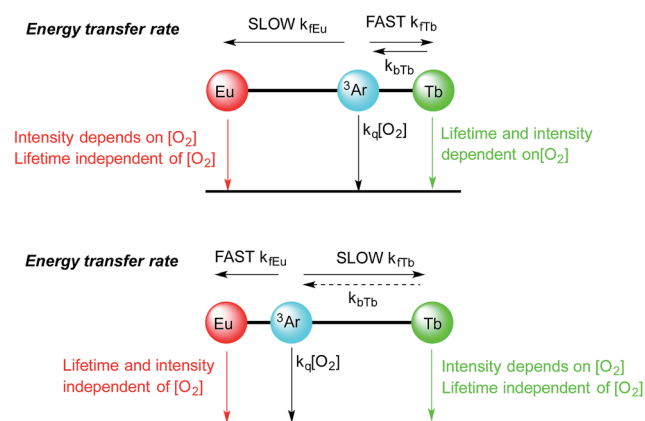
Scheme 2 Cartoons showing the effect of aryl chromophore lanthanide separation on the dependence of oxygen emission, (top) with short Ar–Tb and long Ar–Eu separation, (bottom) with long Ar–Tb and short Ar–Eu separation.
