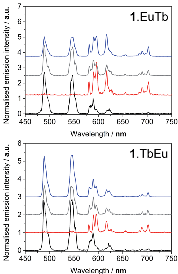
Fig. 3 Emission spectra of 1.EuTb (top) and 1.TbEu (bottom) following excitation at 290 nm (blue), 380 nm (grey), 392 nm (red) and 488 nm (black).
