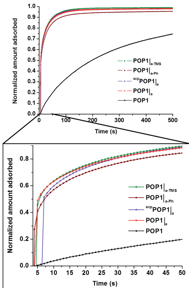
Fig. 6 Time-dependent propane-uptake profiles for POP1, POP1| a , POP1| a-Ph , POP1| a-TMS , and scpPOP1| a at 0.3 bar and 298 K. Data in each profile were normalized to the maximum uptake values at 15 000 s (see complete set of data in the ESI,† Fig. S13).
