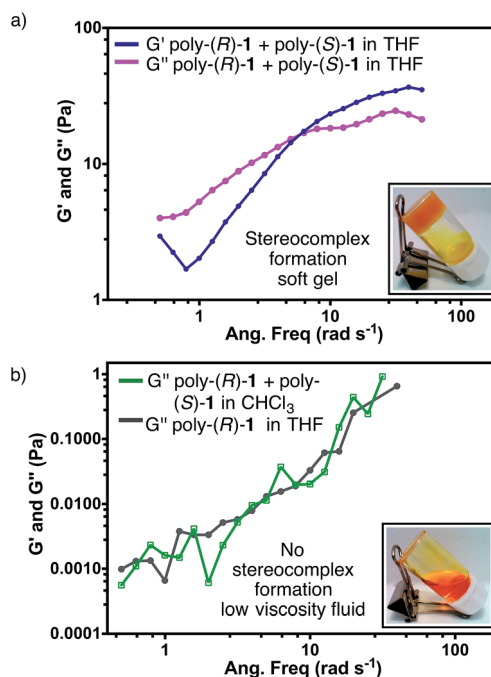
Fig. 7 (a) Rheological studies for the stereocomplex in THF (concentration = 5 \text{ mg mL}^{-1} ). (b) Comparison between the rheological parameter G'' of a mixture of poly-(R)-1 and poly-(S)-1 in \text{CHCl}_3 and of a solution of poly-(R)-1 in THF (concentration = 5 \text{ mg mL}^{-1} ).
