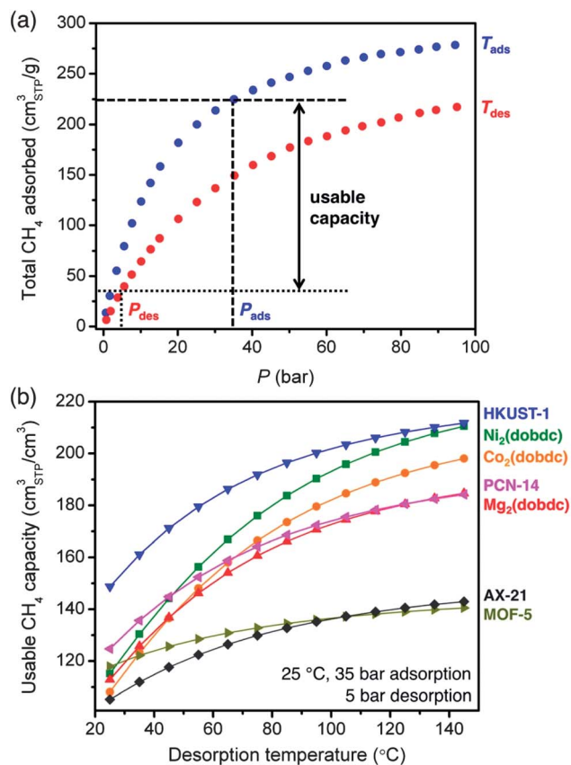
Fig. 6 (a) The usable capacity represents the amount of \text{CH}_4 that can be delivered when discharging from a specific adsorption temperature, T_{\text{ads}} , and pressure, P_{\text{ads}} , to a desorption temperature, T_{\text{des}} , and pressure, P_{\text{des}} . (b) The volumetric usable \text{CH}_4 capacity as a function of desorption temperature for adsorption at 25 °C and 35 bar and desorption at 5 bar.
