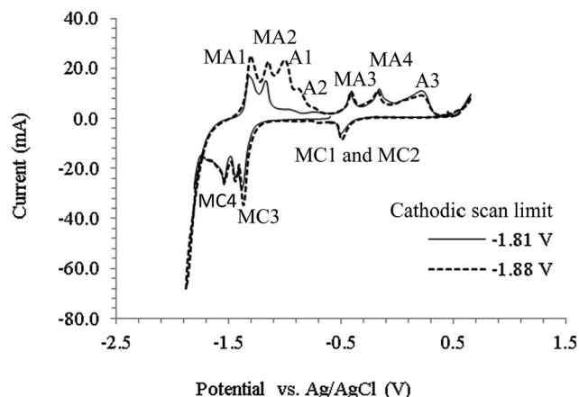
Fig. 3 Cyclic voltammograms obtained using a stainless steel wire working electrode in a molten \text{Li}_2\text{CO}_3\text{-Na}_2\text{CO}_3 electrolyte (molar ratio of 52 : 48) at 627^\circ\text{C} , at a scan rate of 100\text{ mV s}^{-1} , for negative potential limits of -1.81\text{ V} and -1.88\text{ V} . Atmosphere: \text{CO}_2 ; WE diameter: 0.25\text{ mm} ; WE immersion depth: ca. 1.5\text{ cm} ; CE: 6\text{ mm} diameter stainless steel rod; RE: alumina membrane \text{Ag/AgCl} .
