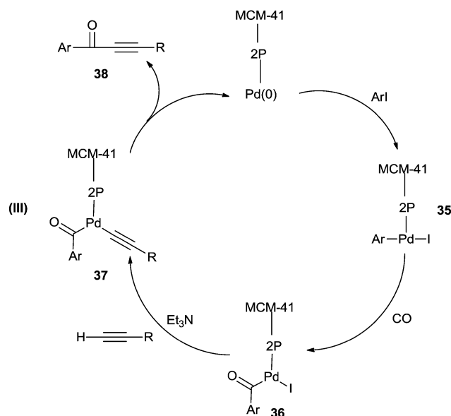
Scheme 57 A plausible mechanism for the MCM-41-2P-Pd(0) catalysed carbonylative Sonogashira coupling of aryl iodides with terminal alkynes.
