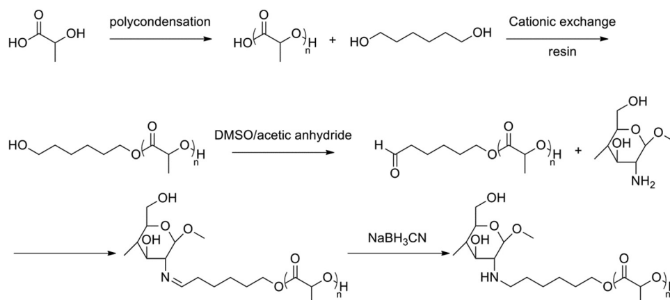
Fig. 9 Synthesis of chitosan- g -oligo(lactic acid). 48
