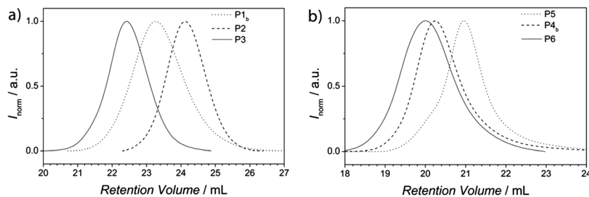
Fig. 1 (a) SEC traces of the polar building block PTEGA ( P2 , dashed line, M_n = 6600 \text{ g mol}^{-1} (PMMA calibration), \mathcal{D} = 1.12 ), the non-polar building block P(S-co-I) ( P1 b , dotted line, M_n = 9200 \text{ g mol}^{-1} (PS calibration), \mathcal{D} = 1.22 ) and the resulting block copolymer P(S-co-I)- b -PTEGA ( P3 , solid line, M_n = 16\,000 \text{ g mol}^{-1} (PS calibration), \mathcal{D} = 1.15 ). (b) SEC traces of the polar building block PTEGA ( P5 , dotted line, M_n = 35\,000 \text{ g mol}^{-1} (PMMA calibration), \mathcal{D} = 1.30 ), the unpolar building block P(S-co-I) ( P4 b , dashed line, M_n = 50\,000 \text{ g mol}^{-1} (PS calibration), \mathcal{D} = 1.36 ) and the resulting block copolymer P(S-co-I)- b -PTEGA ( P6 , solid line, M_n = 68\,000 \text{ g mol}^{-1} (PS calibration), \mathcal{D} = 1.32 ).
