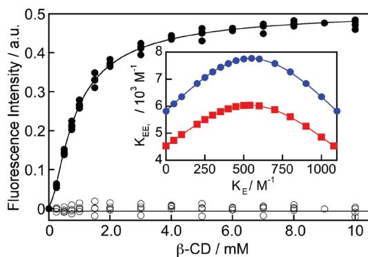
Fig. 4 Dependence of the corrected excimer emission intensity at 390 nm for (R)-NpOH ( 150 \mu\text{M} ) with the \beta\text{-CD} concentration (solid symbols; three independent experiments). The solid line corresponds to the numerical fit of the data using fixed K_E values between 0 and 1100 \text{ M}^{-1} . The residuals between the data and the fit are shown as open symbols. The inset shows the variation of the K_{EE} value as the fixed value for K_E was changed in the numerical fit for (R)-NpOH (blue circles) and (S)-NpOH (red squares). The lines in the inset were included to guide the eye.
