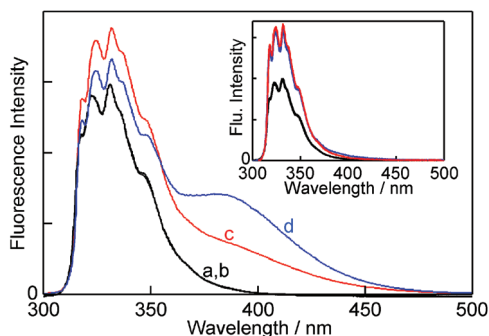
Fig. 2 Fluorescence spectra for ( R )- and ( S )-NpOH (150 \mu M) in the absence (a, b – black; both spectra are superimposed) and presence of 10 mM \beta -CD (c, red ( S )-NpOH; d, blue ( R )-NpOH). The inset shows the fluorescence spectra for ( R )- and ( S )-NpOH (5 \mu M) in the absence (black; both spectra are superimposed) and presence of 10 mM \beta -CD (red ( S )-NpOH and blue ( R )-NpOH; both spectra are superimposed).
