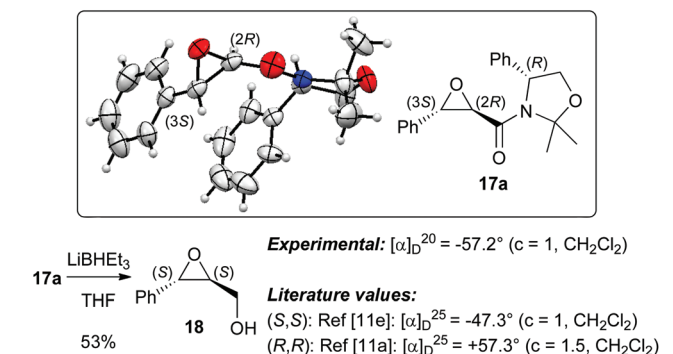
Scheme 6 Molecular structure of 17a and conversion into the known epoxyalcohol 18 .
