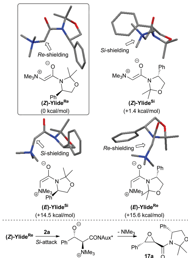
Scheme 7 DFT calculations of the ylide geometry (relative energies given in brackets) and proposed rationale for observed diastereoselectivity. 16
