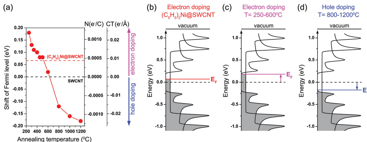
Fig. 6 (a) Fermi level shifts for the \text{NiCp}_2 -filled SWCNTs annealed at 250–1200 °C. Right vertical axes are the corresponding number of electrons transferred to SWCNT's carbon atom N_{\text{total}} ( \text{e}^- per carbon) and the charge transfer density per nanotube length CT ( \text{e}^- \text{\AA}^{-1} ). Dashed horizontal lines denote the values for the pristine and \text{NiCp}_2 -filled SWCNTs. (b–d) Schematics for electron or hole doping of SWCNTs in pristine and annealed \text{NiCp}_2 -filled SWCNTs.
