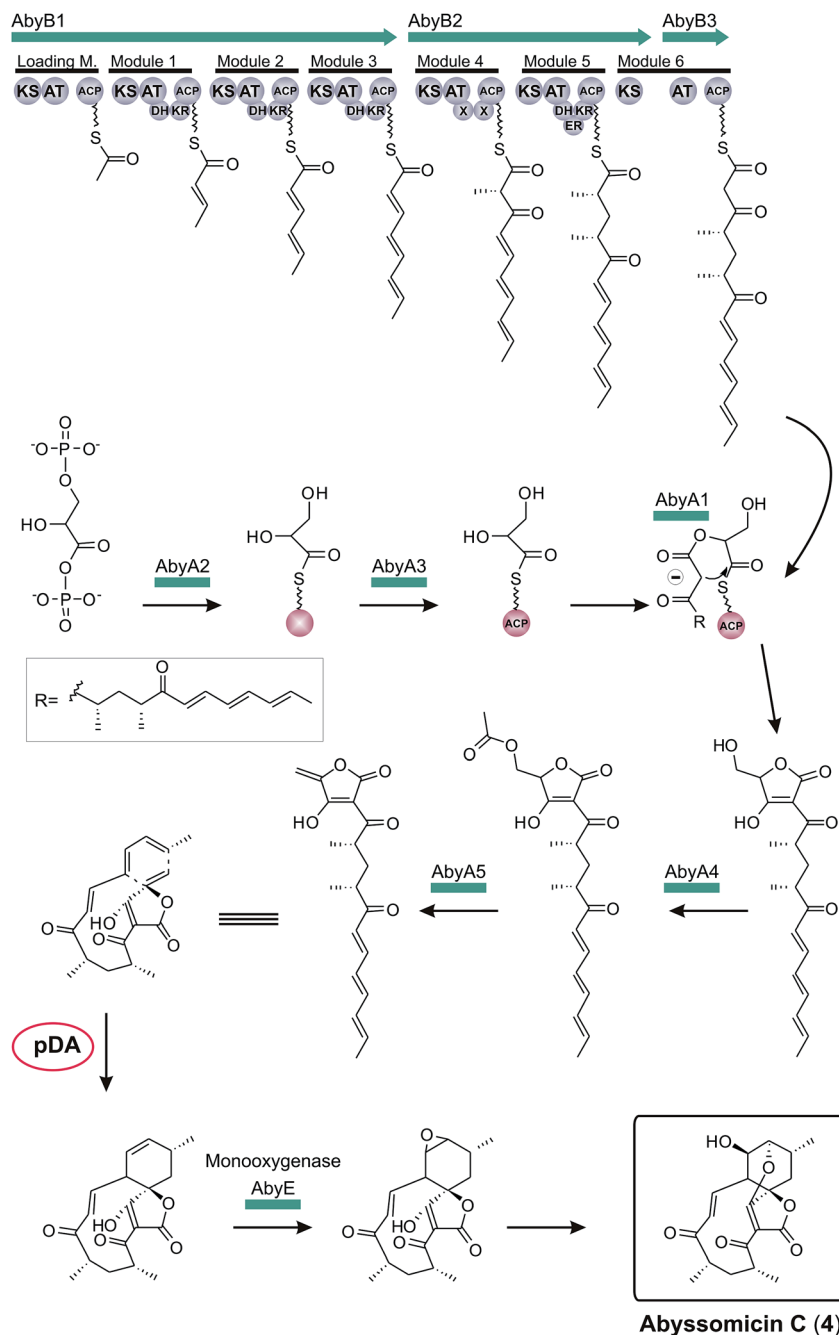
Fig. 10 Model for abyssomicin C ( 4 ) biosynthesis. The multi-enzyme polyketide synthase complex (AbyB1-3) synthesizes the linear polyketide precursor which is then fused to a preactivated and ACP-coupled C 3 -unit, derived from 1,3-bisphosphoglycerate. Tetrone acid maturation steps depicted in this figure are postulated by the authors based on the observation made for the biosynthesis of agglomerin A (AbyA1-5: protein set encoded by the conserved "glycerate utilization operon"). A formal intramolecular Diels-Alder reaction between the exocyclic methylene group of the tetrone acid moiety and a pair of conjugated double bonds in the tail region of the linear polyketide is proposed to take place, thereby generating the abyssomicin macrocycle (pDA = postulated Diels-Alder reaction). Further decoration reactions on the macrocyclic structure yield abyssomicin C ( 4 ) and its derivatives.
