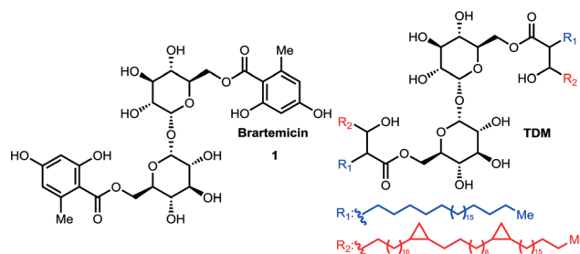
Fig. 1 Chemical structures of brartermicin and trehalose-6,6'-dimycolate = TDM. The side chains of TDM displayed are those of the α-mycolic acid subclass.
