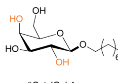
\beta OctylGal 4
