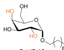
\alpha OctylGal 3
