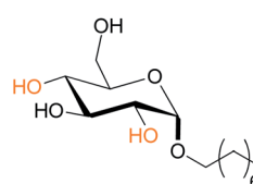
\alpha OctylGlc 5
