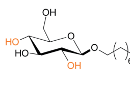
\beta OctylGlc 6
