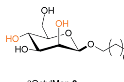
\beta OctylMan 2
