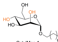
\alpha OctylMan 1
