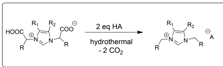
Fig. 1 Hydrothermal decarboxylation of imidazolium zwitterions. R_1, R_2 = \text{H, CH}_3 ; R = amino acid side chain.
