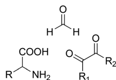
Fig. 1 Hydrothermal decarboxylation of imidazolium zwitterions. R_1, R_2 = \text{H}, \text{CH}_3 ; R = \text{amino acid side chain} .
