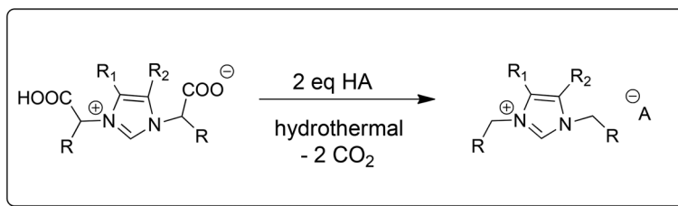
Fig. 1 Hydrothermal decarboxylation of imidazolium zwitterions. R_1, R_2 = \text{H}, \text{CH}_3 ; R = \text{amino acid side chain} .
