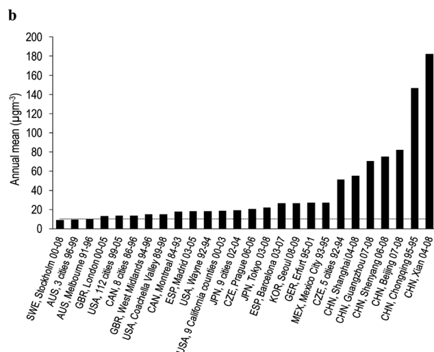
Fig. 2 (a) Literature selection. (b) Selected literature' records of \text{PM}_{2.5} concentrations. Note: Only the annual mean concentrations of the latest exposure year in each city are shown. Three-letter country codes: Australia (AUS), Canada (CAN), China (CHN), Czech Republic (CZE), Germany (GER), Japan (JPN), Korea (KOR), Mexico (MEX), Spain (ESP), Sweden (SWE), United Kingdom (GBR), and United States (USA). The dotted line represents the WHO annual AQG of 10 \mu\text{g m}^{-3} for \text{PM}_{2.5} .
