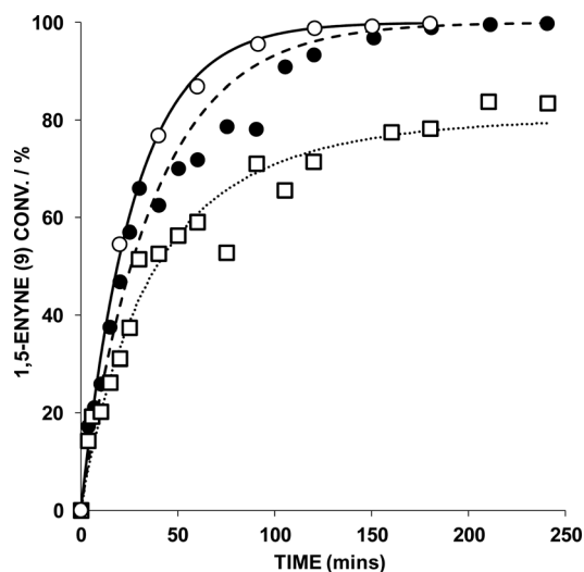
Fig. 4 Effect of 1,5-enyne concentration [9] in a reaction mediated by AuBr 2 (N-phthal)(I I' Pe) (1 mol%), AgOTf (1 mol%), in DCE at 25 °C (key: ○ = 0.1 M 9; ● = 0.2 M 9; □ = 0.5 M 9). 1,5-Enyne conversion monitored by GC analysis – each sample point was quenched by addition of ( n -Bu) 4 NBr. The kinetic curves were fitted using Dynafit™.
