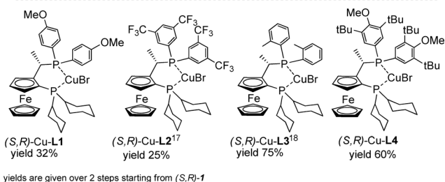
Scheme 1 General procedure for the synthesis of copper complexes of rev-Josiphos derivatives.
