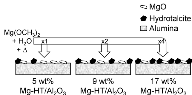
Scheme 1 Growth of hydrotalcite coating over alumina support.
