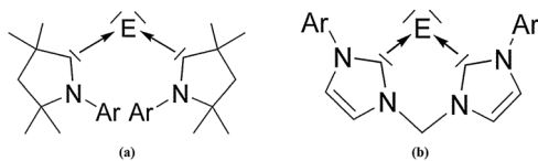
Fig. 15 Schematic representation of the silylones and germlylones E(CAAC)_2 and E(NHC-NHC) ( E = Si, Ge ) which have been isolated. 54,55
