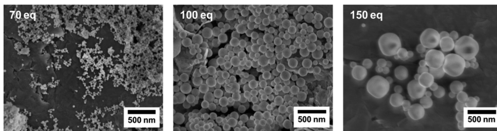
Fig. 4 SEM images of Zr- fum MOF samples synthesised with various concentrations of the modulator (as given in the images) in a water-based synthesis at 43 °C (ZrCl 4 /H 2 fum/formic acid/H 2 O 1:3:x:1074).
