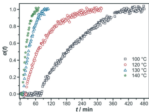
Fig. 5 Extent of crystallisation \alpha plotted against time t . Crystallisation curves measured for syntheses of Zr- fum MOF in DMF-based systems by varying the temperature T (ZrCl 4 /H 2 fum/formic acid/DMF in molar ratios of 1:3:70:500).
