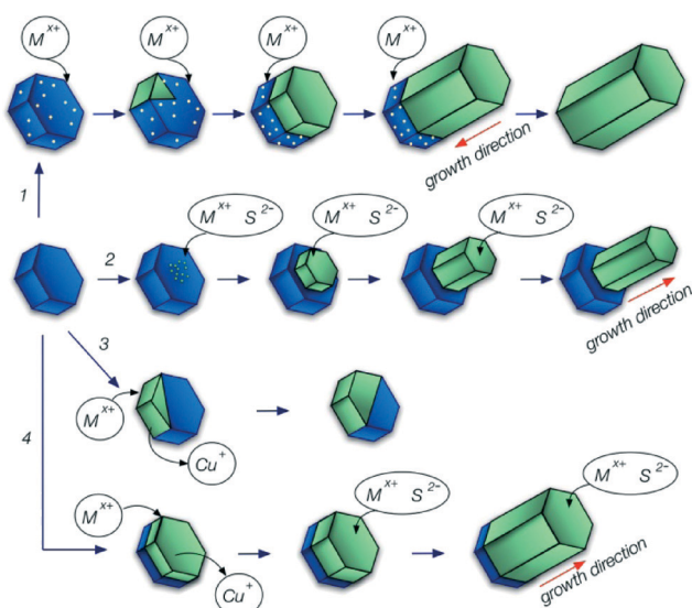
Scheme 1 Possible growth mechanisms of copper sulphide based hybrid nanostructures by reaction with other cations M^{x+} ( In^{3+} , Ga^{3+} , Zn^{2+} , Sn^{2+} , Cd^{2+} , Pb^{2+} , or Mn^{2+} ). Pathway 1: copper sulphide plays the role of a catalyst. Dissolution of M^{x+} in the copper sulphide phase leads to the nucleation of a second semiconductor material. The growth takes place at the interface between the two phases. In some cases the copper sulphide phase gradually disappears. Pathway 2: copper sulphide plays the role of a seed for heterogeneous nucleation of another material on its surface; the resulting particles are always copper sulphide containing heterostructures. Pathway 3: partial cation exchange leading to the formation of copper sulphide containing heterostructures. Pathway 4: partial cation exchange followed by seeded growth.
