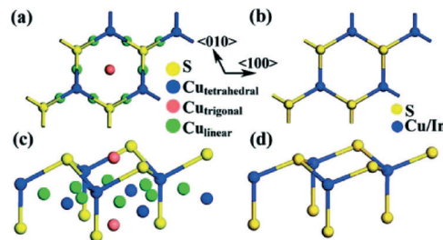
Fig. 1 Crystal structures of (a) hexagonal chalcocite Cu_2S and (b) hexagonal CuInS_2 with a zone axis of \langle 001 \rangle . Crystal structures of (c) hexagonal chalcocite Cu_2S and (d) hexagonal CuInS_2 viewed from another angle. Reprinted with permission from J. Am. Chem. Soc. , 2009, 131 , 4962–4966. Copyright (2009) American Chemical Society.
