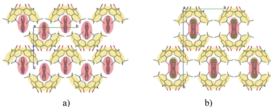
Fig. 1 The two most often occurring packing arrangements of the inclusion compounds of 5,11,17,23-tetra- tert -butyl-25,26,27,28-tetrahydroxycalix[4]arene in the space groups of a) P2/n and P4/n with 1:1 stoichiometry (MUBHUM, P4/n ) as well as b) P4/nnc with 2:1 stoichiometry (QUSGOA).
