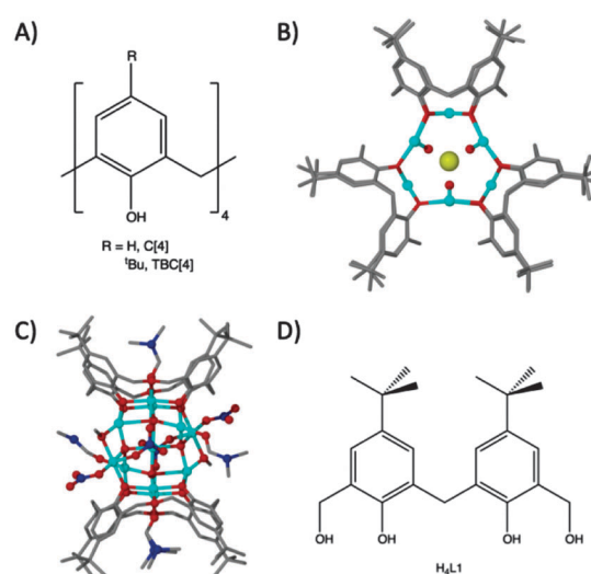
Fig. 1 (A) General calix[4]arene framework. (B) Tri-capped trigonal prismatic [\text{Cu}^{\text{II}}_9(\text{TBC}[4])_3]\text{Cl}_2 cluster, viewed down the face of the prism. 4 (C) \text{Cu}_{11} cluster formed with tetrahomodioxacalix[4]arene. 12 (D) Schematic of \text{H}_4\text{L}_1 .
