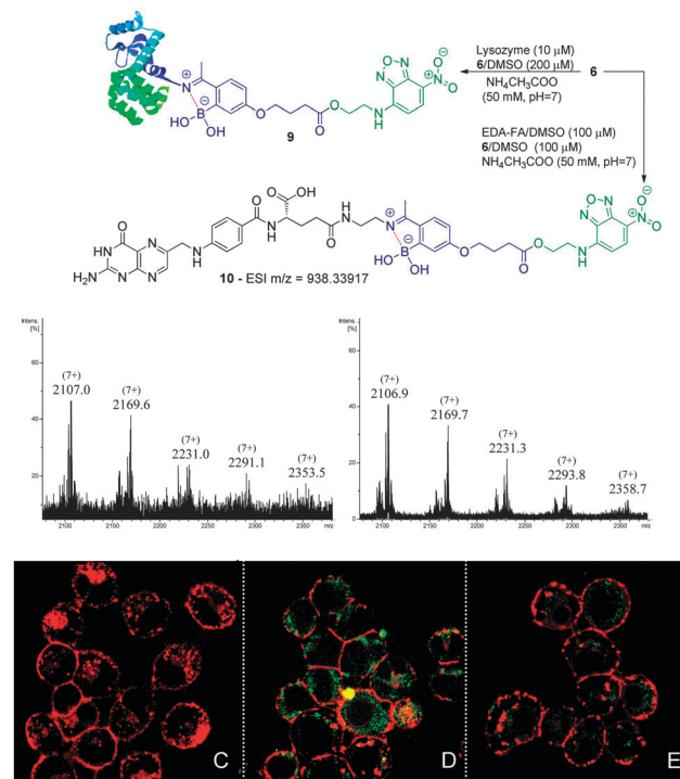
Scheme 4 Reaction of lysozyme (10 \mu\text{M} ) with 6 (200 \mu\text{M} ) in acetate buffer (50 mM, pH 7) at room temperature. Zoom of the (7+) charge state of the ESI-FTICR-MS spectra after 30 min and 2 h of reaction. Reaction of EDA-FA (100 \mu\text{M} ) with compound 6 (100 \mu\text{M} ) in acetate buffer (50 mM, pH 7) to obtain 10 as confirmed by HRMS. NCI-H460 (C) and NCI-H460 without (D) and with pre-treatment with EDA-FA (E) were incubated with compound 10 . The procedure is described in Scheme 3.
