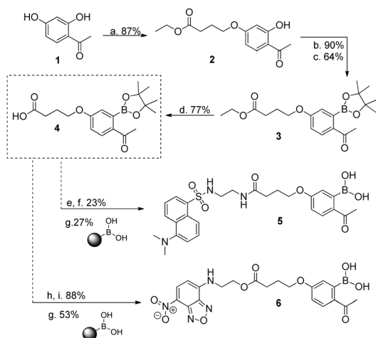
Scheme 2 (a) Ethyl 4-bromobutyrate, \text{K}_2\text{CO}_3 , NaI, acetone, reflux, 20 h; (b) \text{PhNTf}_2 , TEA, DMF, rt, 2 h; (c) (\text{Bpin})_2 , \text{PdCl}_2(\text{dppf}) , \text{NaCH}_3\text{CO}_2 , dioxane, 95 °C, 4 h; (d) TFA, \text{H}_2\text{O} , 90 °C, 3 h; (e) NHS-OH, DCC, THF, rt, 16 h; (f) 2-dansylaminoethylamine, THF, rt, 2 h; (g) \text{CH}_3\text{CN}:\text{HCl} (1 M) (9 : 1), 20 h, rt, 20 h; (h) DMAP, DCC; DCM, 0 °C, 0.5 h; (i) 4-ethanolamine-7-nitrobenzofurazan, DCM, rt, 22 h. UV spectra: see ESI† for compounds 5 and 6 .
