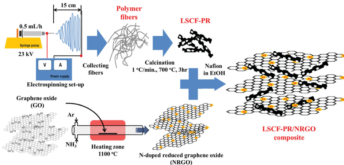
Fig. 33 Schematic presentation of the preparation route leading to perovskite-graphene composite with special morphology. Reproduced with permission from ref. 667. Copyright Elsevier 2014.
