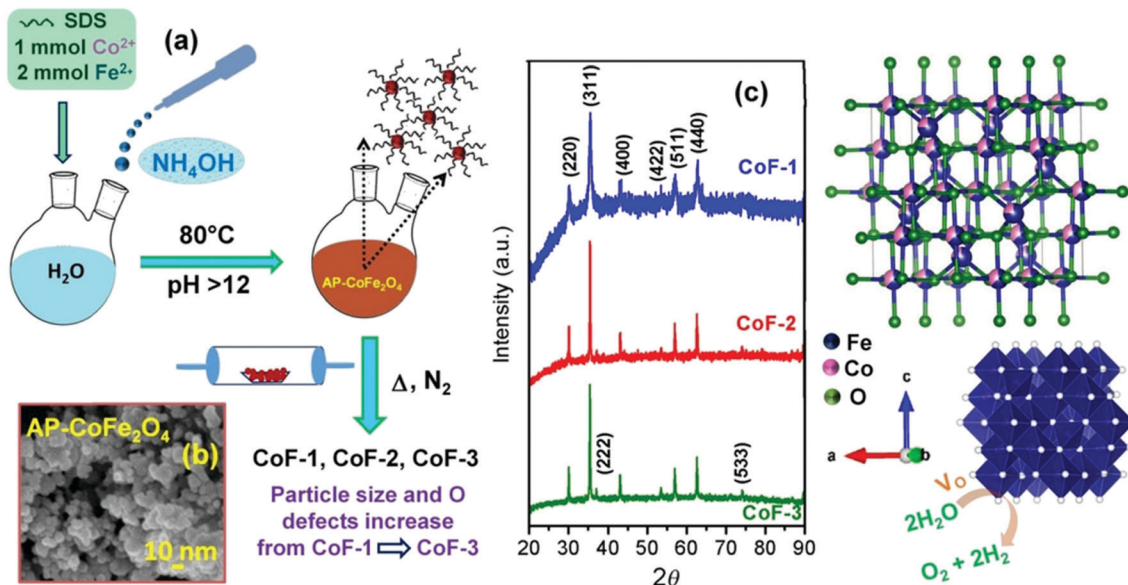
Fig. 47 (a) Schematic illustration of the formation of AP- \text{CoFe}_2\text{O}_4 through the coprecipitation method followed by thermal treatment under \text{N}_2 to obtain CoF-1, CoF-2, and CoF-3. (b) Field-emission (FE) SEM image of AP- \text{CoFe}_2\text{O}_4 . (c) XRD patterns of CoF-1, CoF-2, and CoF-3 NPs. Reproduced with permission from ref. 811. Copyright Wiley 2020.
