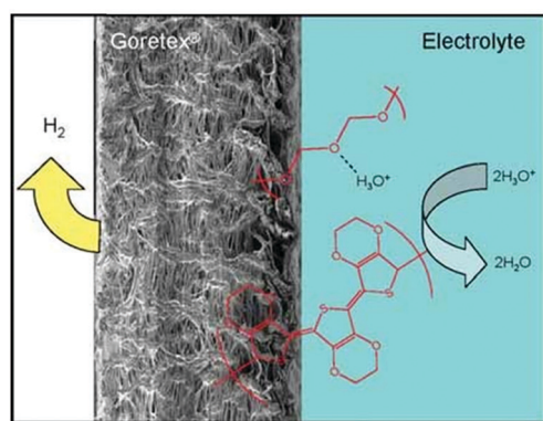
Fig. 94 Schematic of PEDOT-based HER electrode (left side). Long-term performance of PEDOT-PEG on Goretex/Au in 1 M \text{H}_2\text{SO}_4 under \text{N}_2 at -0.35 V vs. SCE. Reproduced with permission from ref. 1339. Copyright 2010 Wiley.
