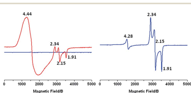
Fig. 4 X-band EPR of: (left) 16 mM [\text{Co}^{\text{III}}(\text{NH}_3)_5\text{Cl}]^{2+} and 0.80 mM complex \mathbf{1-OH}_2 in a 4 : 1 \text{H}_2\text{O} : \text{CH}_3\text{CN} solvent mixture before (blue) and after (red) 2 min illumination with 450 nm light. (Right) 1.65 mM solution of complex \mathbf{1-OH}_2 after addition of 2 eq. \text{H}_2\text{O}_2 . The weak resonance at g = 4.28 is due to the ubiquitous S = 5/2 \text{Fe}^{\text{III}} species.
